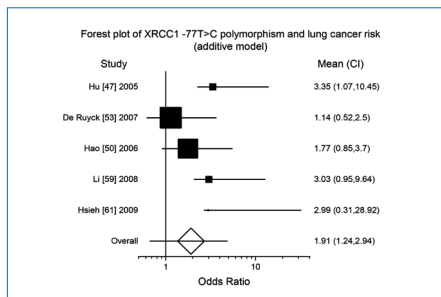
Forest Plot
