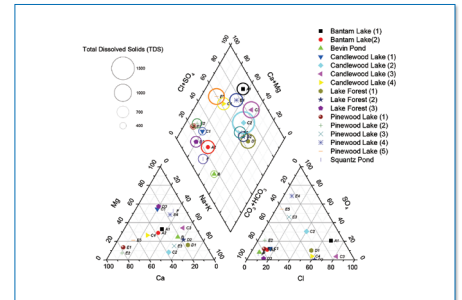
Piper Diagram
